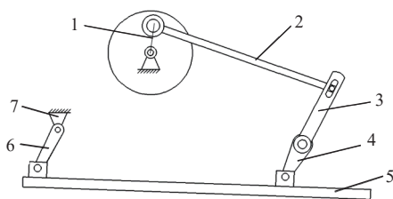
a. Vibrating sieve drive mechanism model
