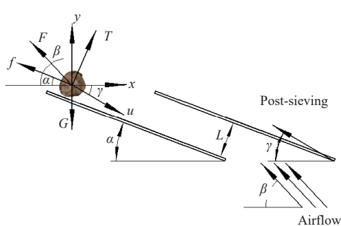
a. The vibrating sieve accelerates upward and the seeds slide downward
