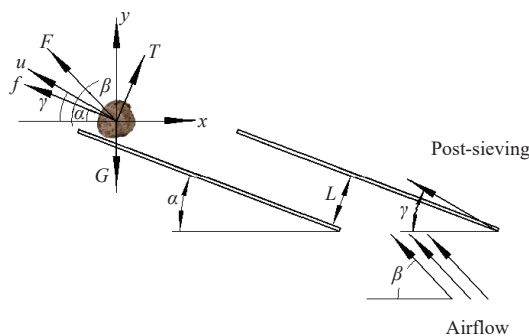
b. The vibrating sieve decelerates downward and the seeds slide downward
