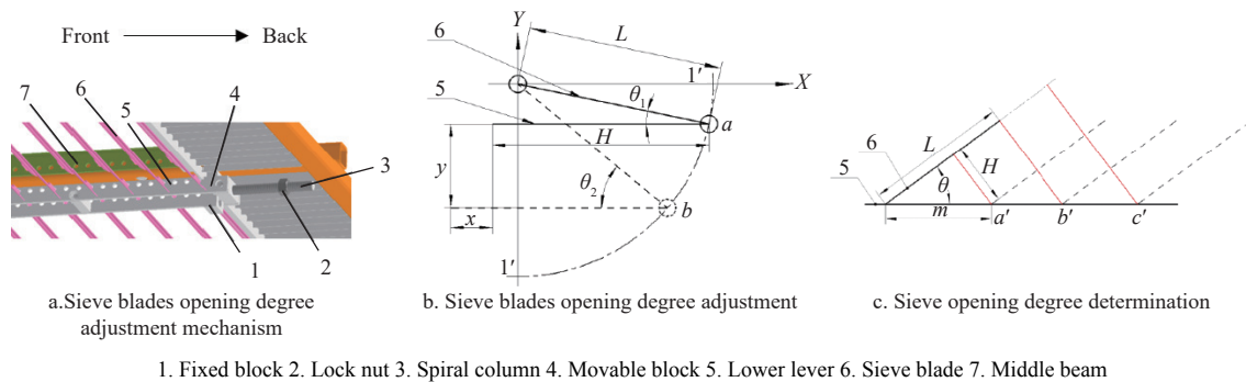
Figure 7 Vibrating screen blade opening adjustment process
