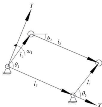
b. Movement sketch of the mechanism
